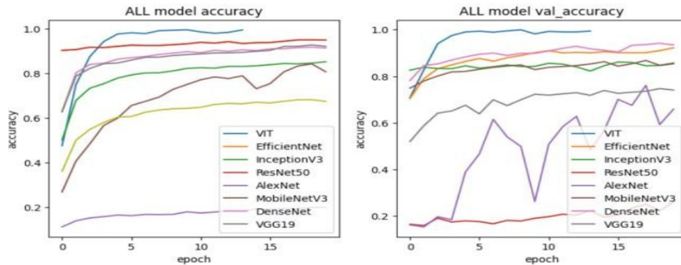
Figure 3: All Model Training and validation accuracy curves
