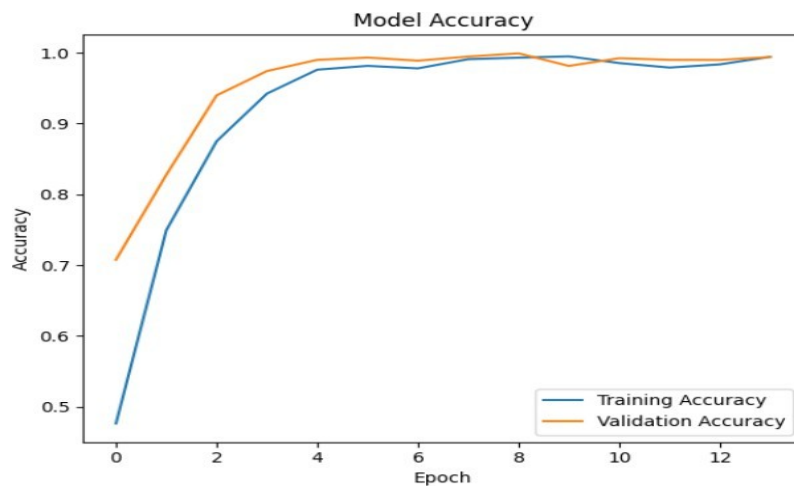
Figure 5: Training and validation accuracy curves for the Vision Transformer model
